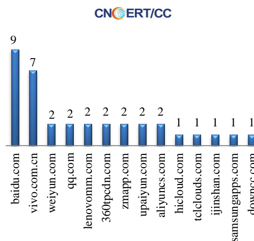
CNCERT Coordinated Mobile Phone Application Stores to Handle Mobile Malware (Nov 6-Nov 11)
