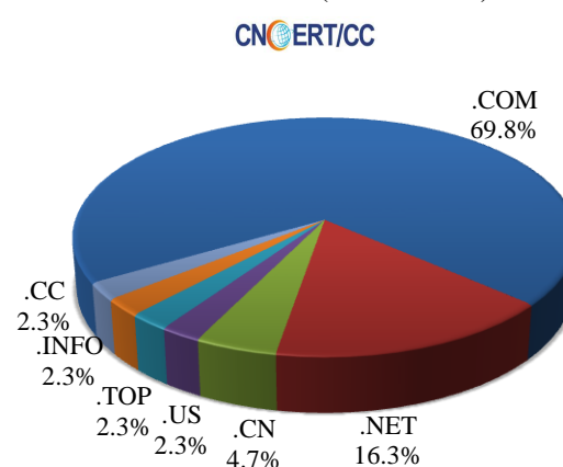
TLD Distribution of the Malware-hosting Websites' Domains (Nov 6-Nov 11)
